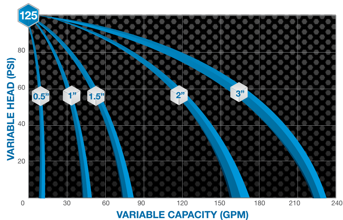
Composite Performance Curve
