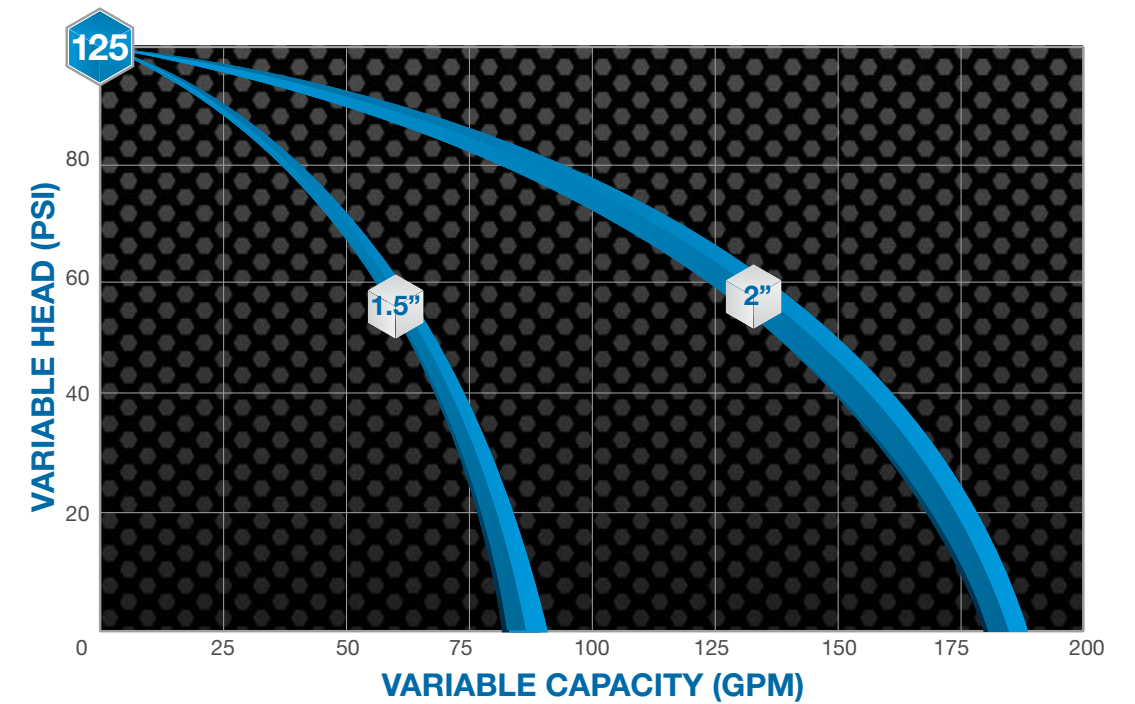
Composite Performance Curve
