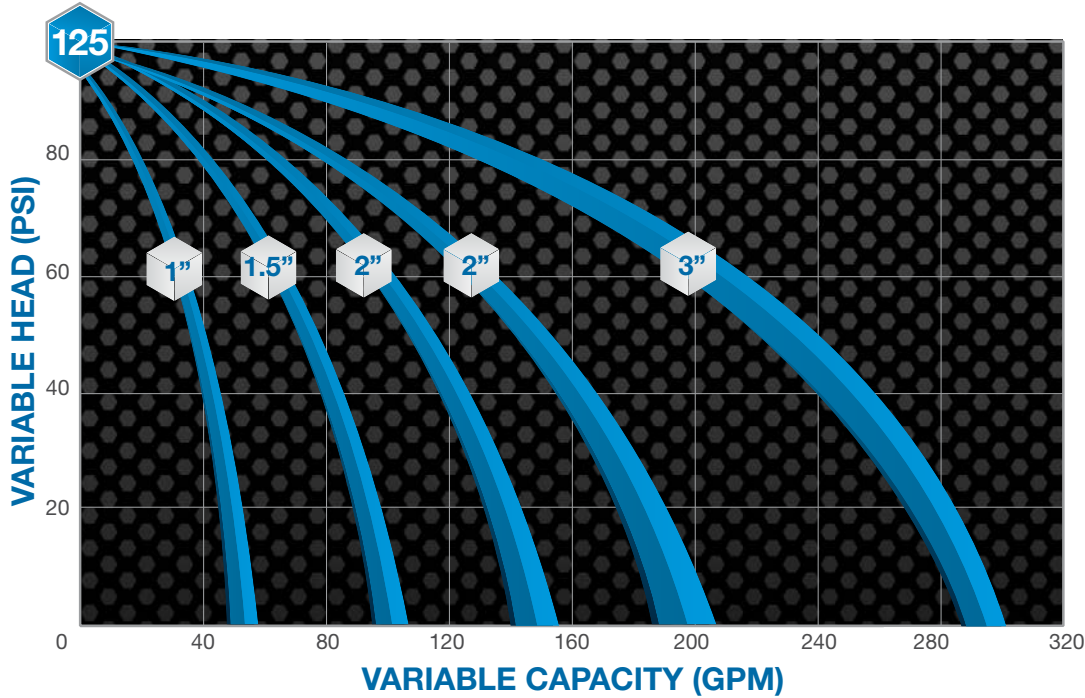
Composite Performance Curve
